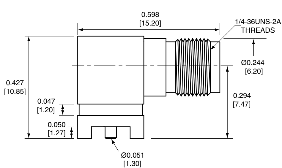
SIDE VIEW
