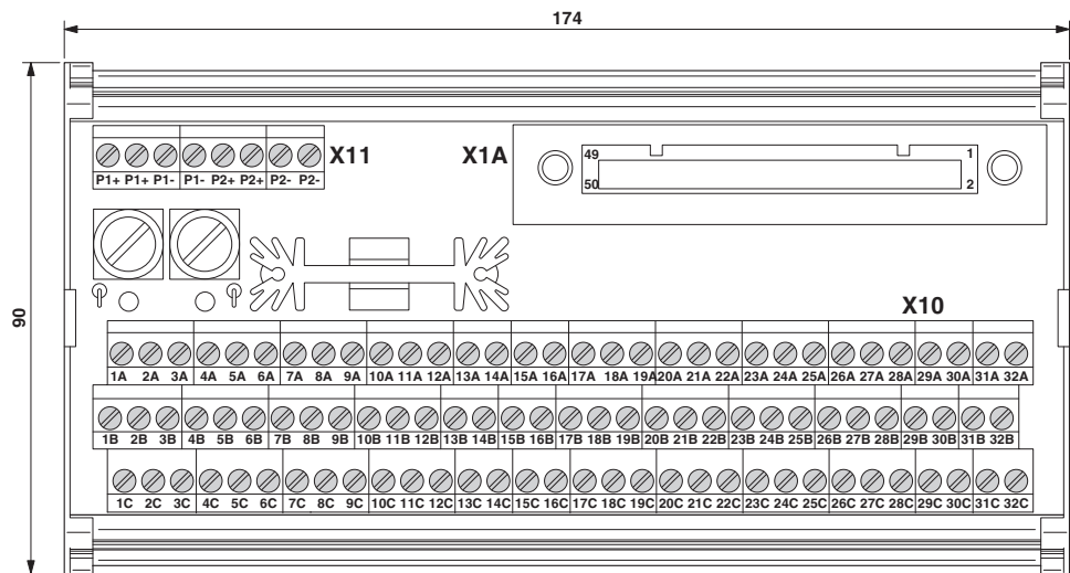
Dimensioned drawing
