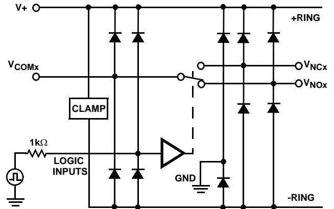
FIGURE 9. OVERVOLTAGE PROTECTION
