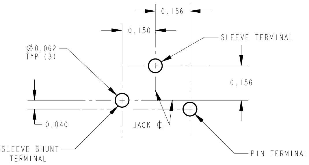
PC BOARD LAYOUT SCALE: 1 = .250
