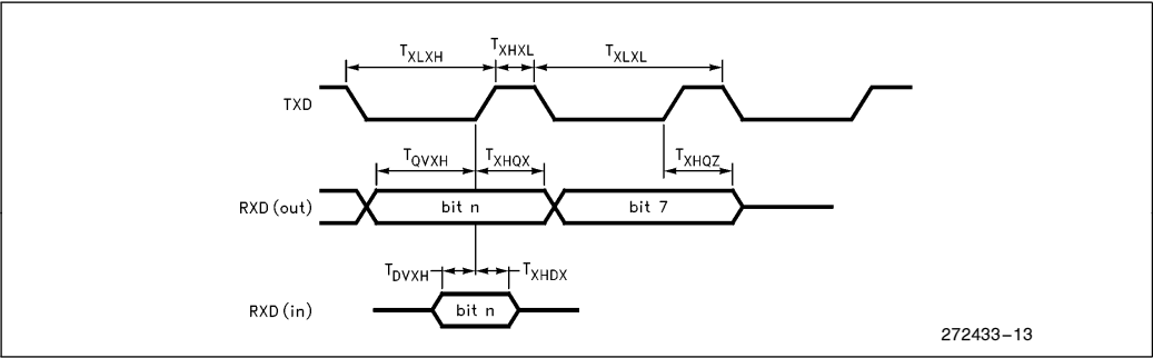
Figure 11. Relative Signal Waveform
