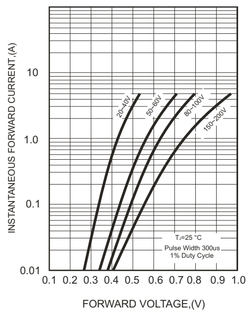
FIG.2-TYPICAL FORWARD CHARACTERISTICS
