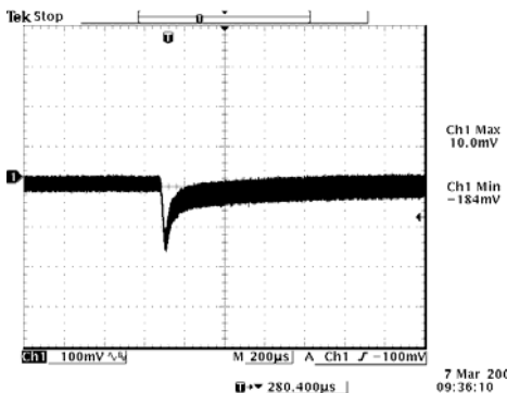
Vout=12 V 50% to 100% Load Transients
