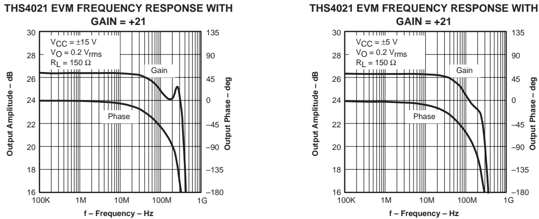
Figure 1–3. THS4021 EVM Frequency Response With Gain = +21
