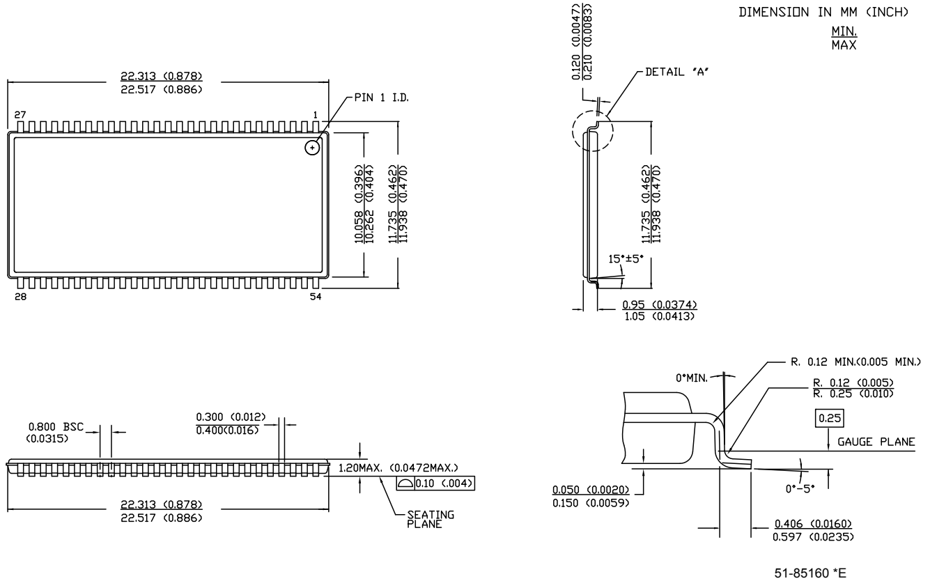
Figure 18. 54-pin TSOP II (22.4 × 11.84 × 1.0 mm) Package Outline, 51-85160
