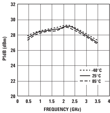
Figure 16. P1dB vs. Temperature and Frequency at optimum OIP3.
