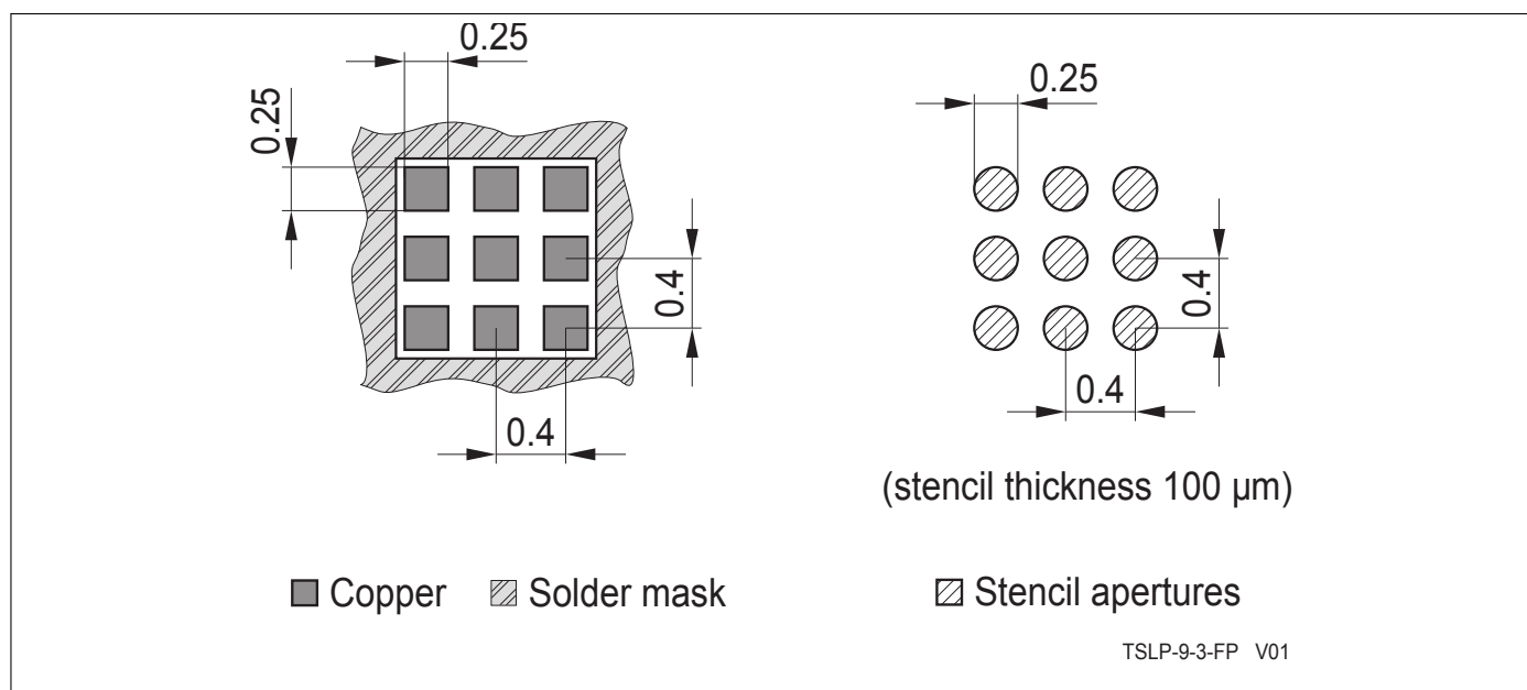
Figure 4: Footprint TSLP-9-3
