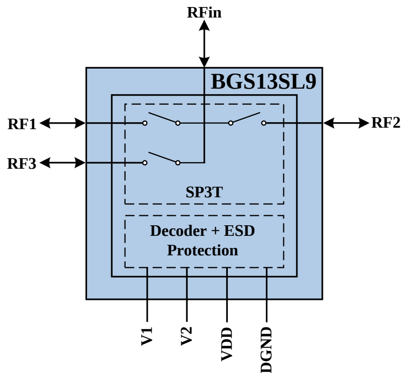
Figure 1: BGS13SL9 Block Diagram
