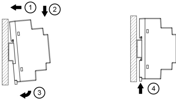
Fig. 2.1 Mounting
