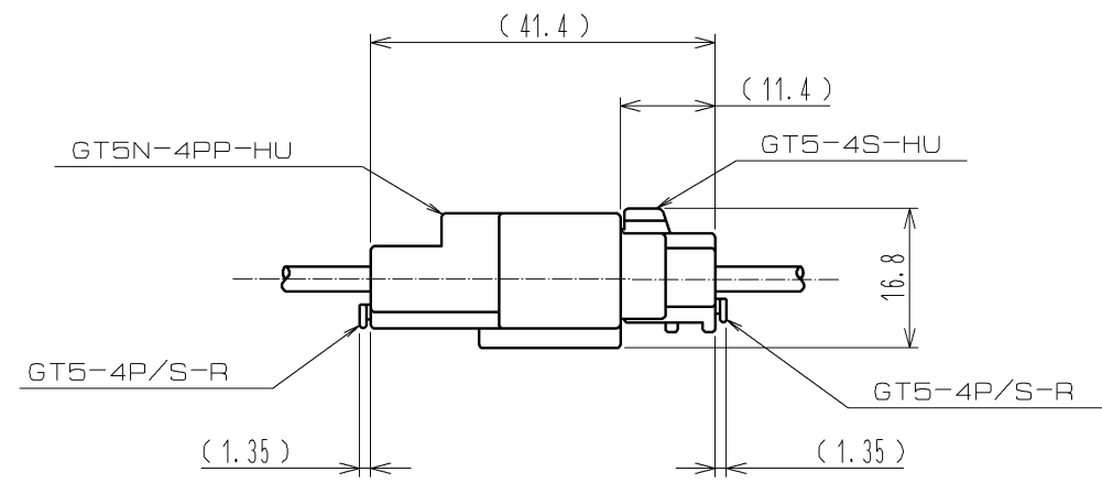
MATED CONNECTORS
