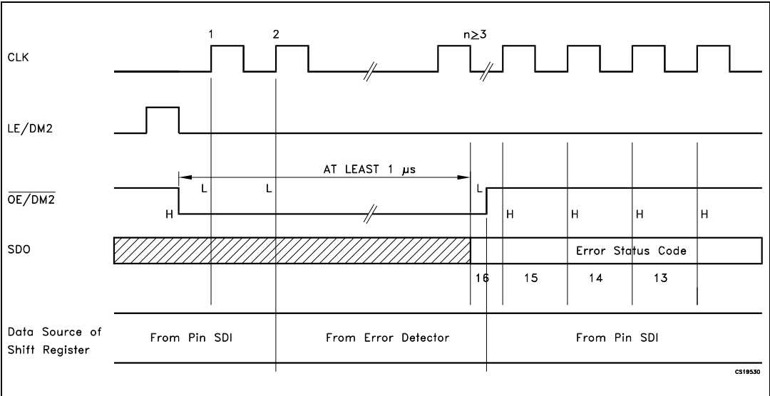
Figure 16. Detection diagram
