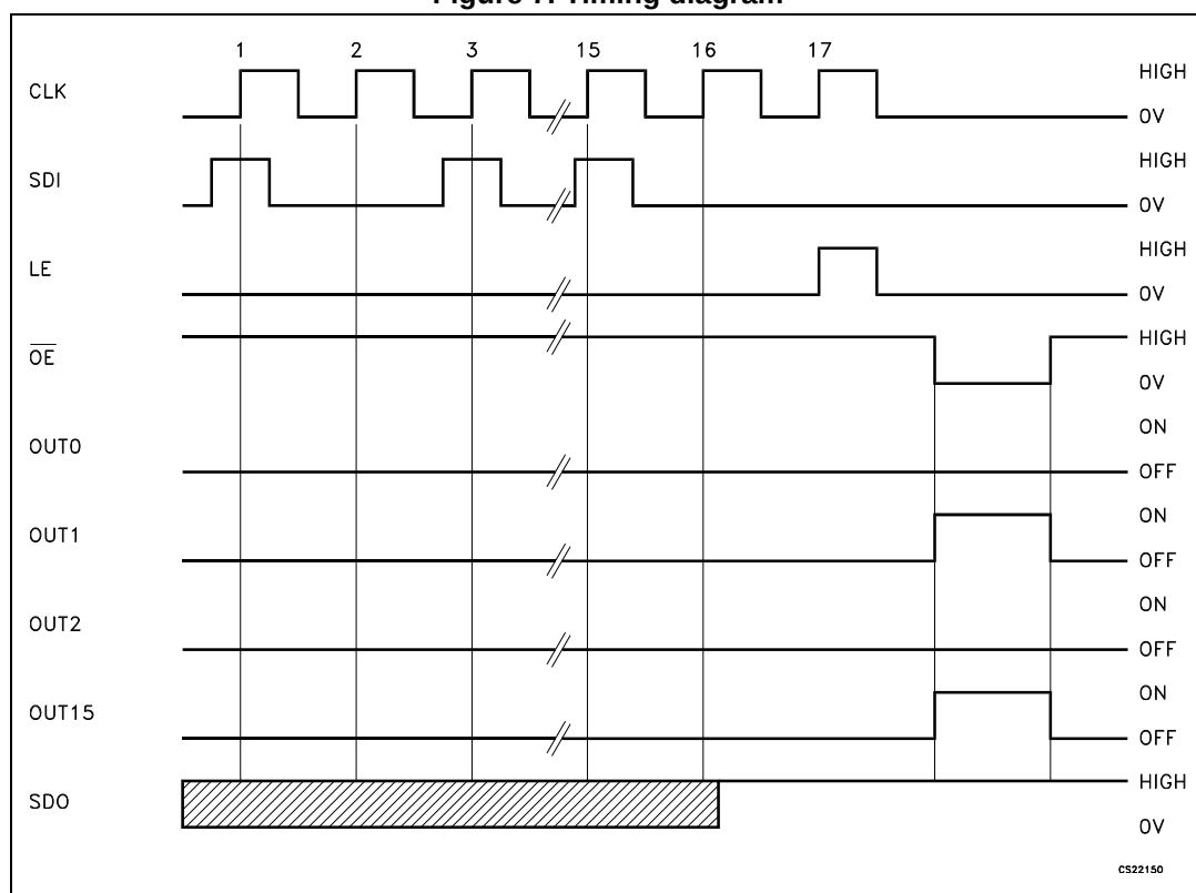
Figure 7. Timing diagram
