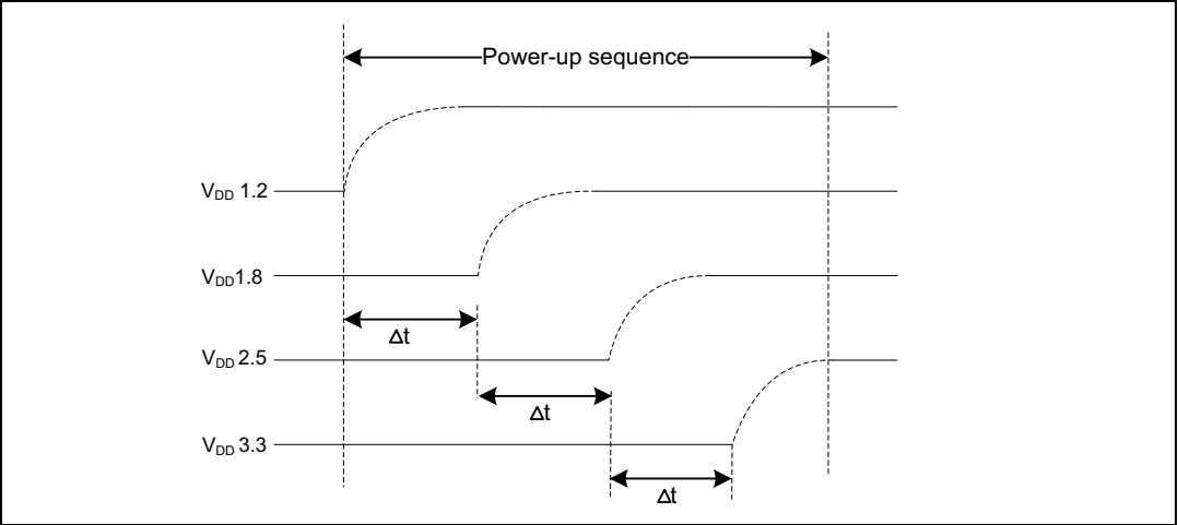
Figure 4. Power-up sequence
