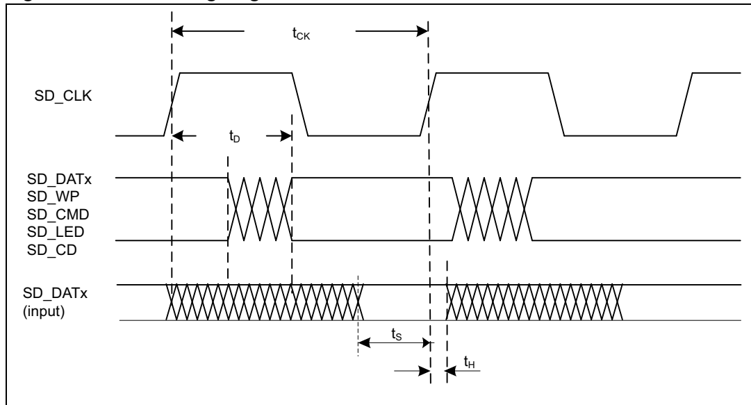
Figure 18. SDIO timing diagram
