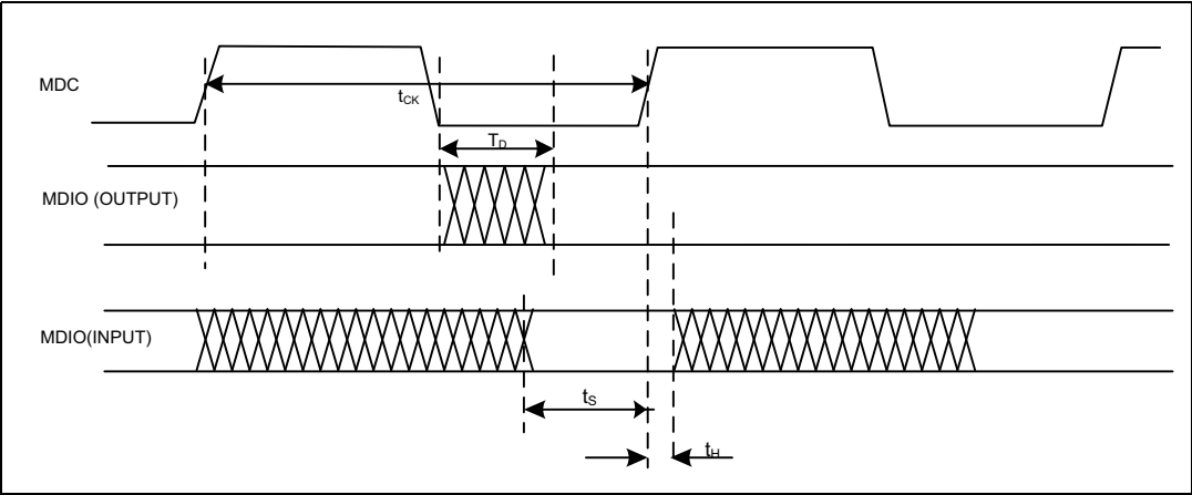
Figure 21. MDC waveforms
