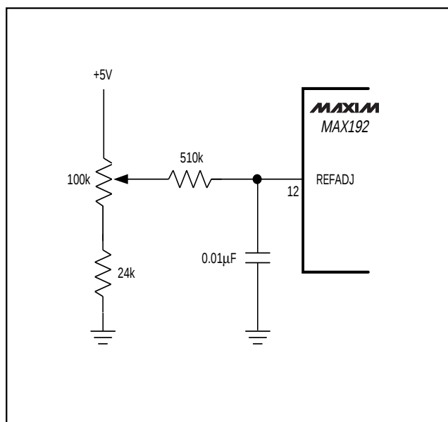
Figure 17. Reference-Adjust Circuit
