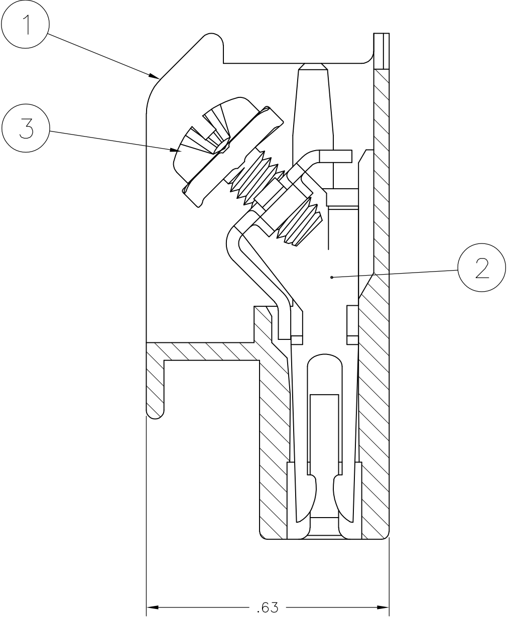
SECTION H-H
