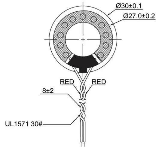
BOTTOM VIEW
