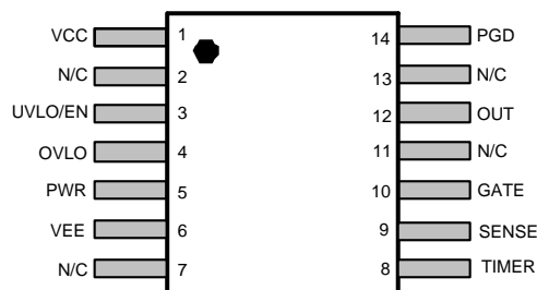
Figure 3. Top View 14-Lead SOIC
