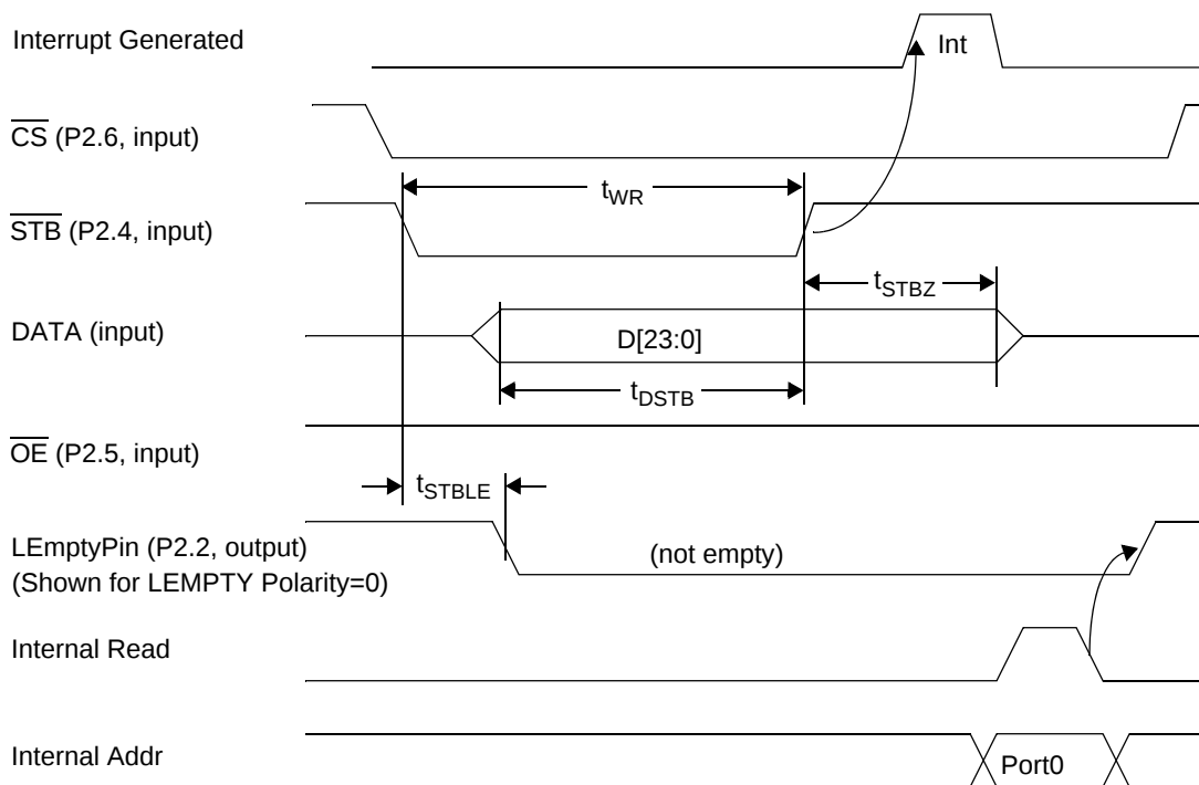
Figure 52. HAPI Write by External Device to USB Microcontroller
