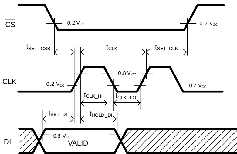
Figure 6. SPI Timing
