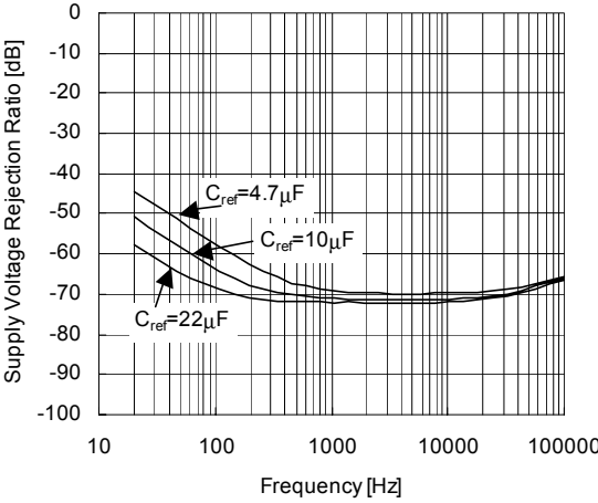
Supply Voltage Rejection Ratio vs. Frequency V_+ = 9V , V_{ripple} = 100mV , R_g = 600\Omega , T_a = 25^\circ C
