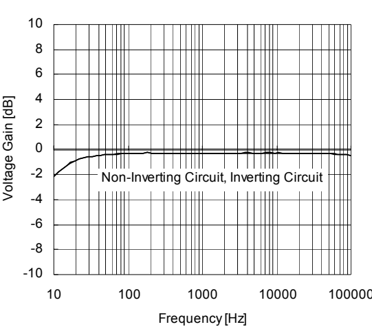
Voltage Gain vs. Frequency V_+ = 9V , V_{in} = 1V_{rms} , T_a = 25^\circ C
