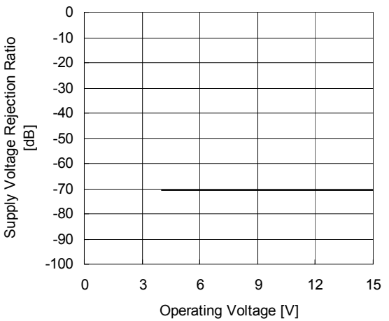
Supply Voltage Rejection Ratio vs. Operating Voltage V_{ripple} = 100mV , f = 100Hz , R_g = 600\Omega , T_a = 25^\circ C
