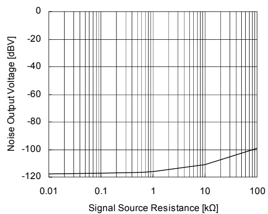
Noise Output Voltage vs. Signal Source Resistance V+=9V, Ta=25°C, A-Weighted
