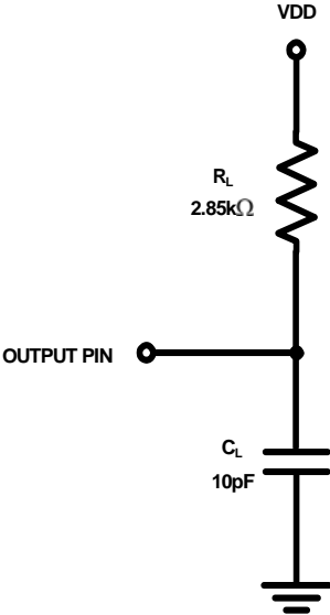
FIGURE 4. EQUIVALENT LOAD CIRCUIT
