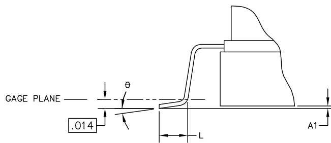
DETAIL "G"
