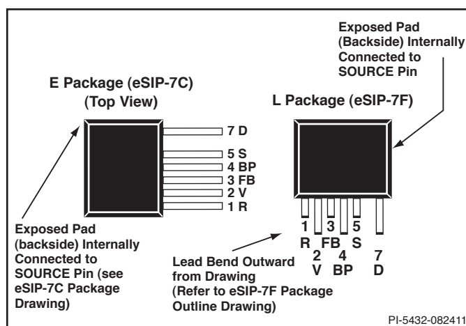
Figure 4. Pin Configuration.
