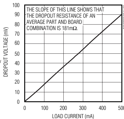
OUT4 REGULATOR DROPOUT VOLTAGE vs. LOAD CURRENT
