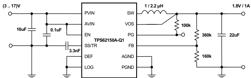
Figure 33. 1.8V/1A Power Supply
