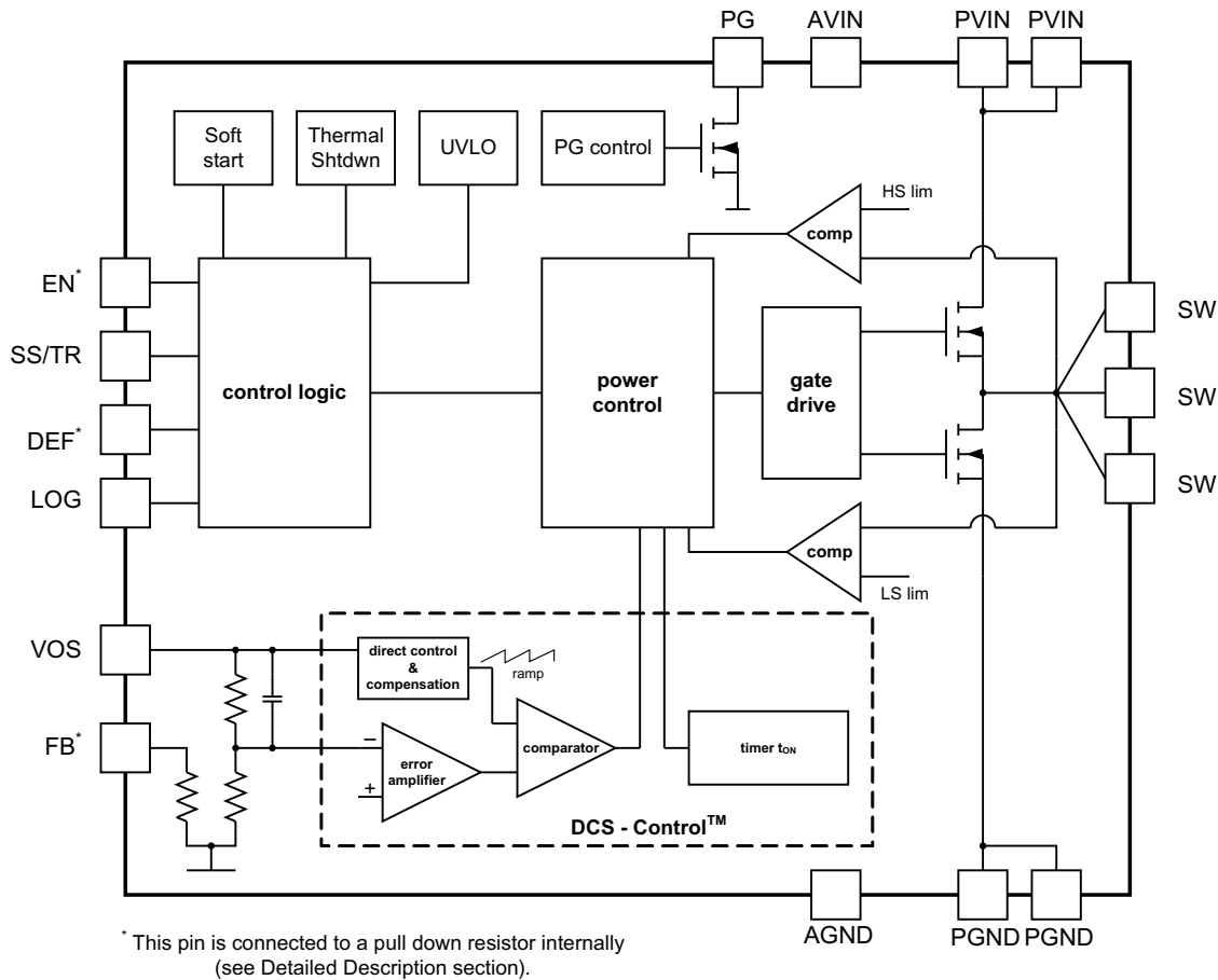
Figure 15. TPS62153A-Q1 (5V Fixed Output Voltage)
