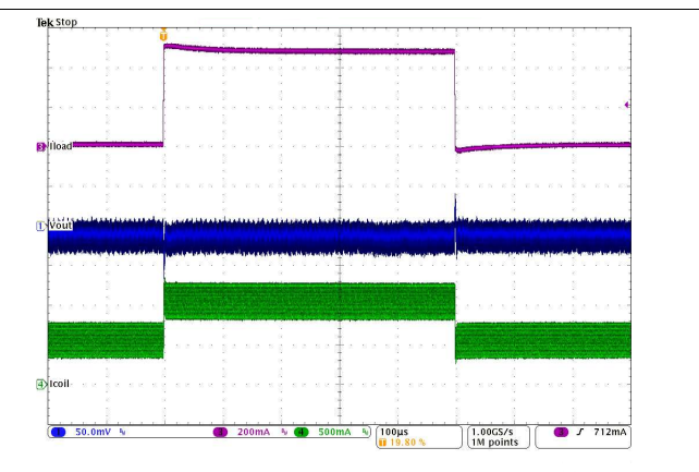
Figure 22. Load Transient Response (0.5 to 1 to 0.5 A)
