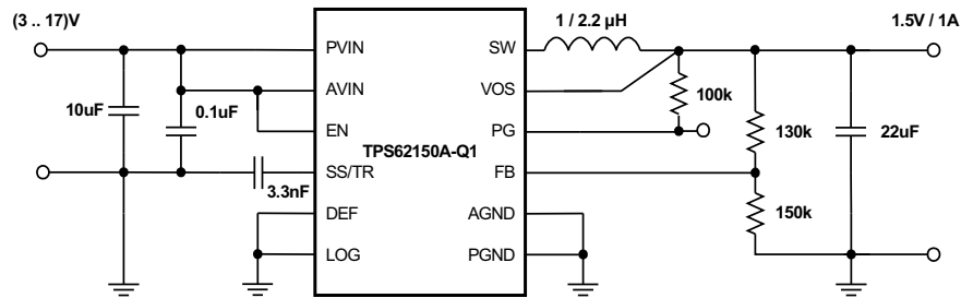
Figure 34. 1.5V/1A Power Supply
