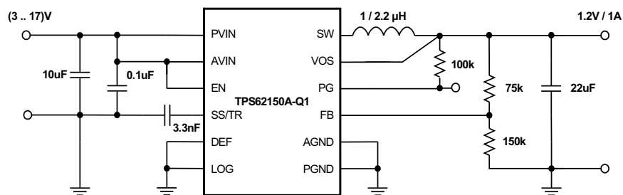
Figure 35. 1.2V/1A Power Supply
