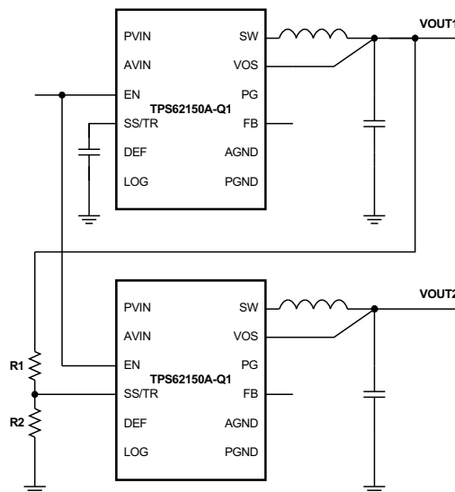
Figure 18. Sequence for Ratiometric and Simultaneous Startup
