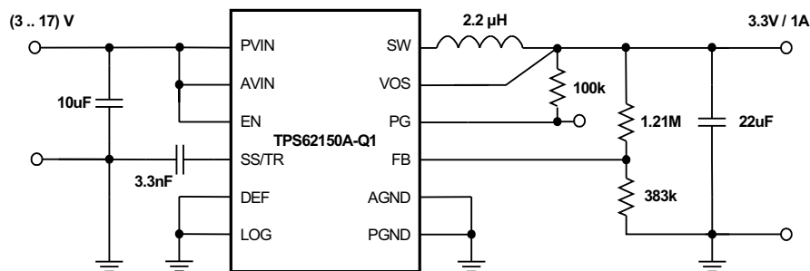
Figure 16. Typical Schematic for 3.3V Step-Down Converter
