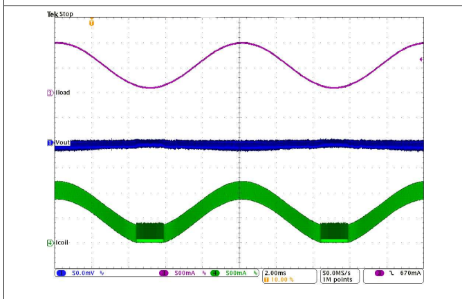
Figure 21. PWM-PSM-Transition
