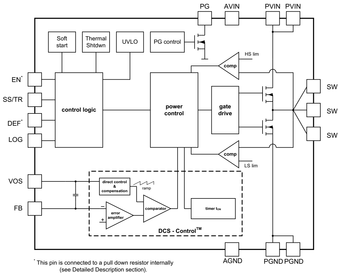
Figure 14. TPS62150A-Q1 (Adjustable Output Voltage)
