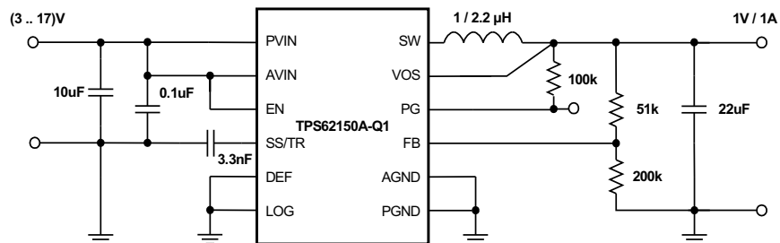
Figure 36. 1V/1A Power Supply
