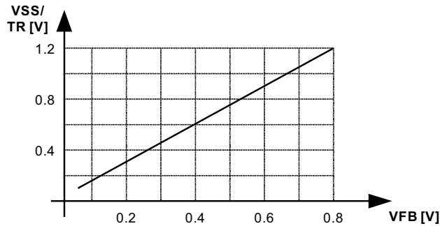
Figure 17. Voltage Tracking Relationship
