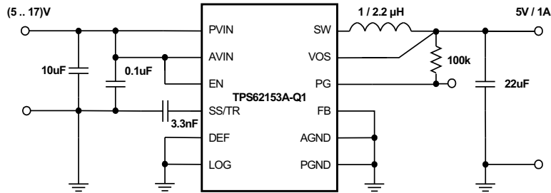
Figure 30. 5V Power Supply Using TPS62153A-Q1 Fixed V_{OUT} Version
