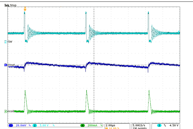
Figure 20. Typical Operation in Power Save Mode ( I_{OUT} = 10mA )
