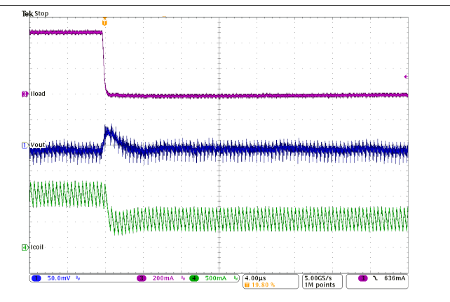
Figure 24. Load Transient Response of Figure 22, Falling Edge
