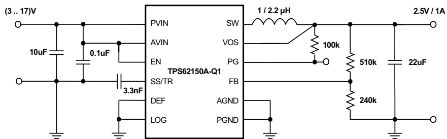
Figure 32. 2.5V/1A Power Supply
