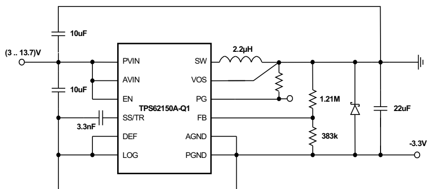
Figure 28. -3.3V Inverting Power Supply
