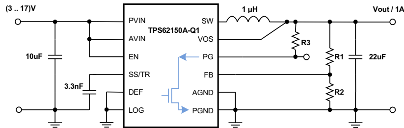
Figure 29. Output Discharge Using PG Pin
