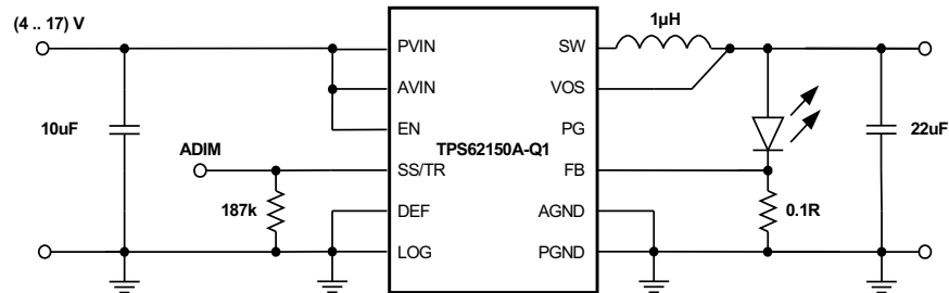
Figure 27. Single Power LED Supply
