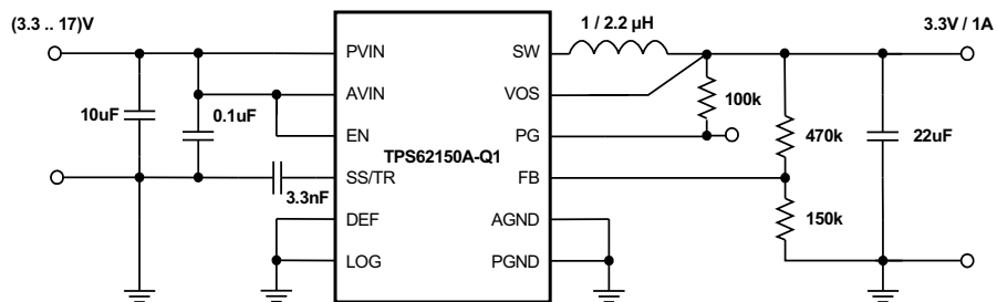
Figure 31. 3.3V/1A Power Supply
