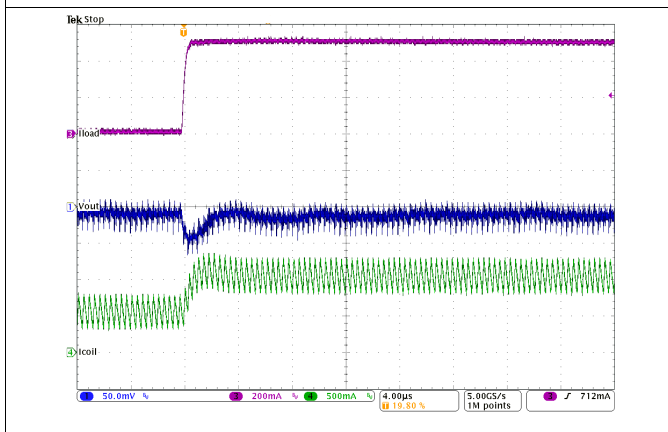
Figure 23. Load Transient Response of Figure 22, Rising Edge
