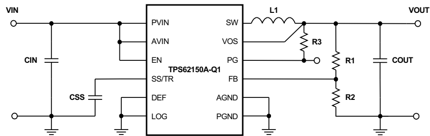
Figure 13. Measurement Setup
