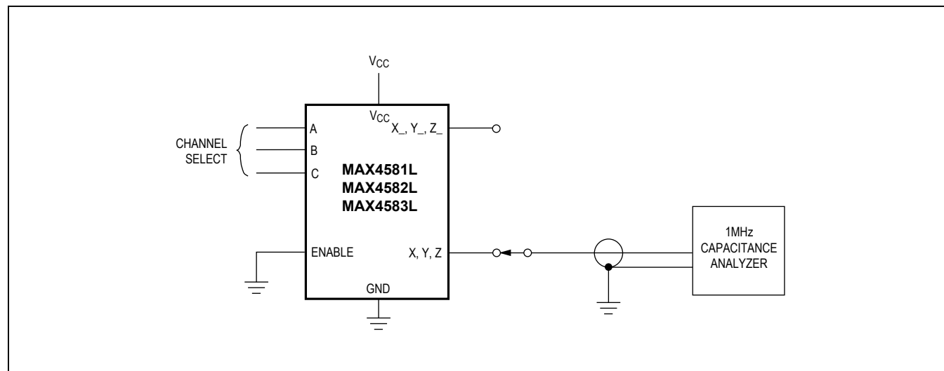
Figure 5. NO/COM Capacitance
