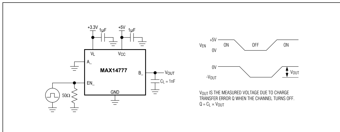
Figure 7. Charge Injection
