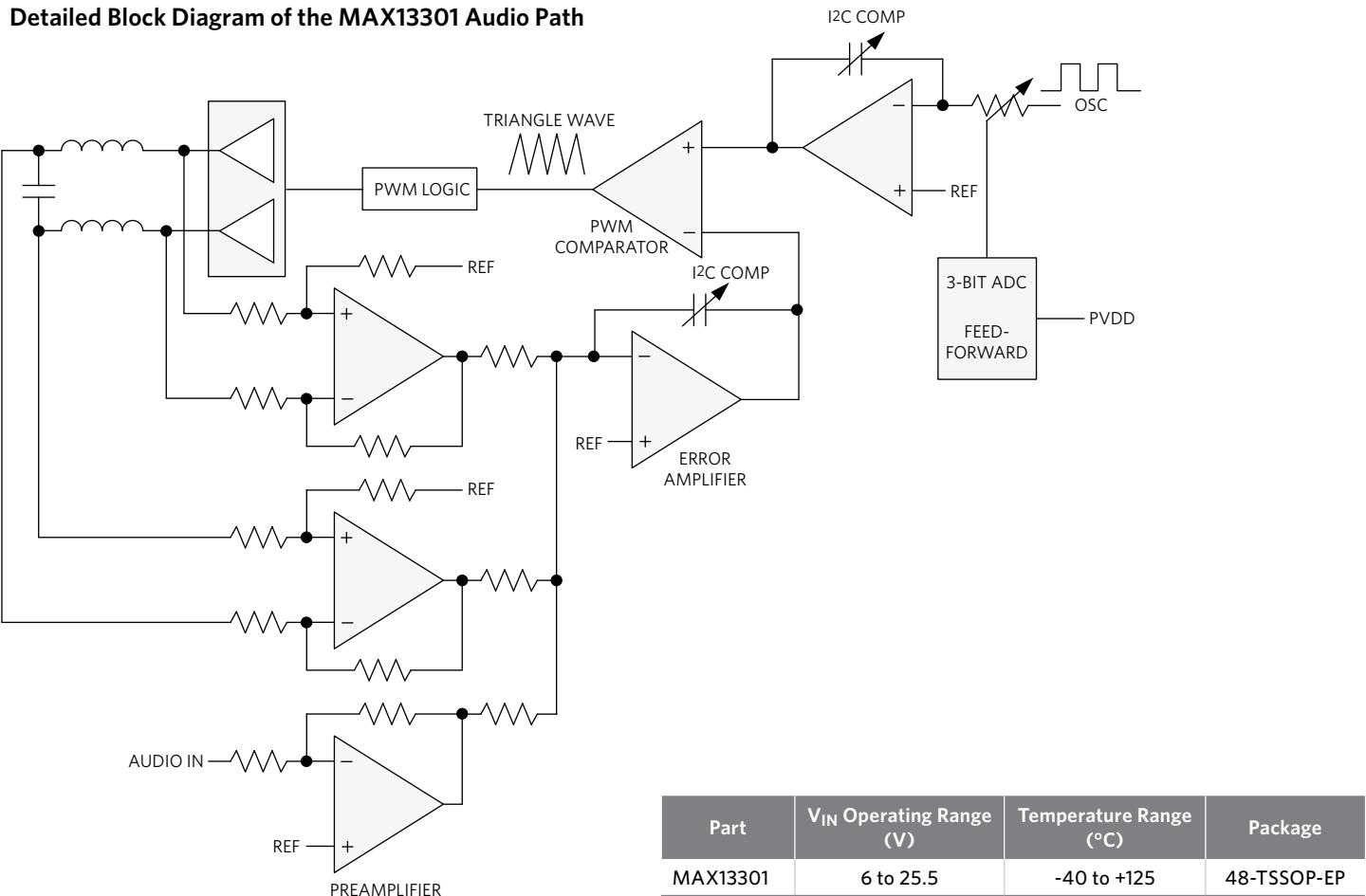
Detailed Block Diagram of the MAX13301 Audio Path
