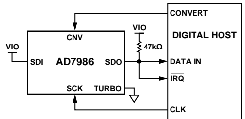
Figure 27. \overline{CS} Mode, 3-Wire with Busy Indicator Connection Diagram (SDI High)
