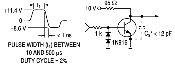
Figure 4. t_{\text{off}} Circuit – 100 mA
