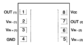
TS482IQT - DFN8
