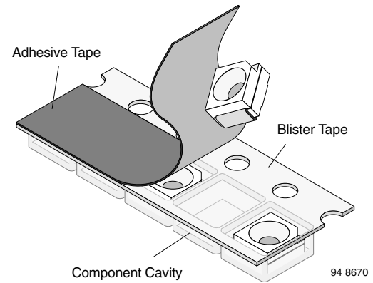
Figure 10. Blister Tape
