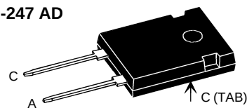
TO-247 AD
