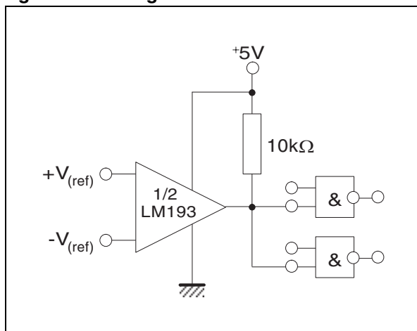
Figure 9. Driving CMOS
