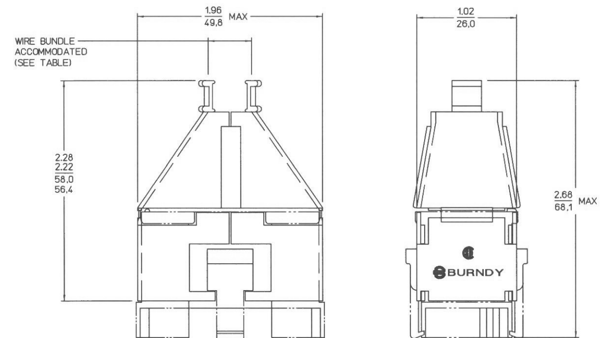
HOOD CAT. NO. SMS/SMV36H-1 (ASSEMBLED TO SMS/SMV36P-1)
