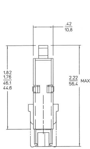
HOOD CAT. NO. SMS/SMV3H-1 (ASSEMBLED TO SMS/SMV3P-1)
