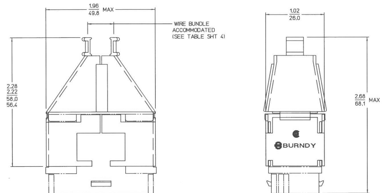
HOOD CAT. NO. SMS/SMV36H-1 (ASSEMBLED TO SMS/SMV36R-10)
