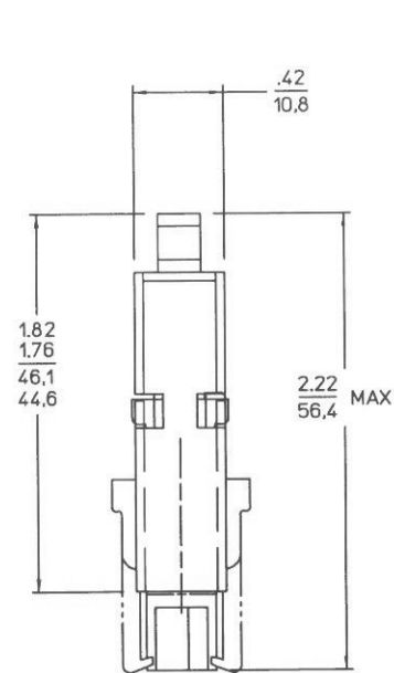
HOOD CAT. NO. SMS/SMV2H-1 (ASSEMBLED TO SMS/SMV2P-1)
