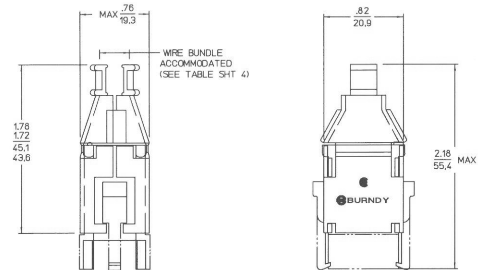
HOOD CAT. NO. SMS/SMV9H-1 (ASSEMBLED TO SMS/SMV9P-1)
