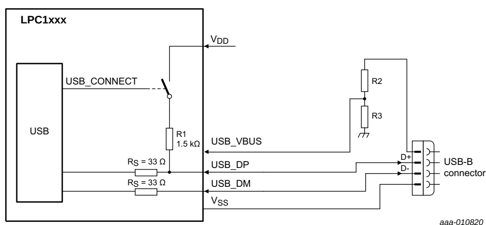
Fig 38. USB interface on a self-powered device where USB_VBUS = 5 V
