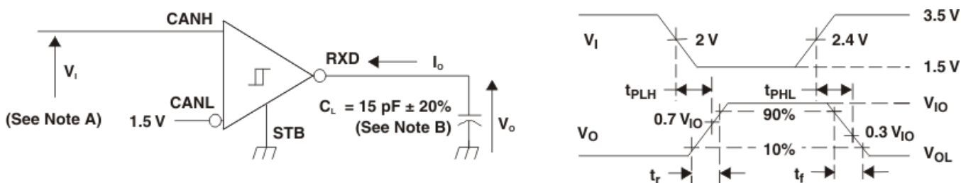
Figure 11. Receiver Voltage and Current Definitions
