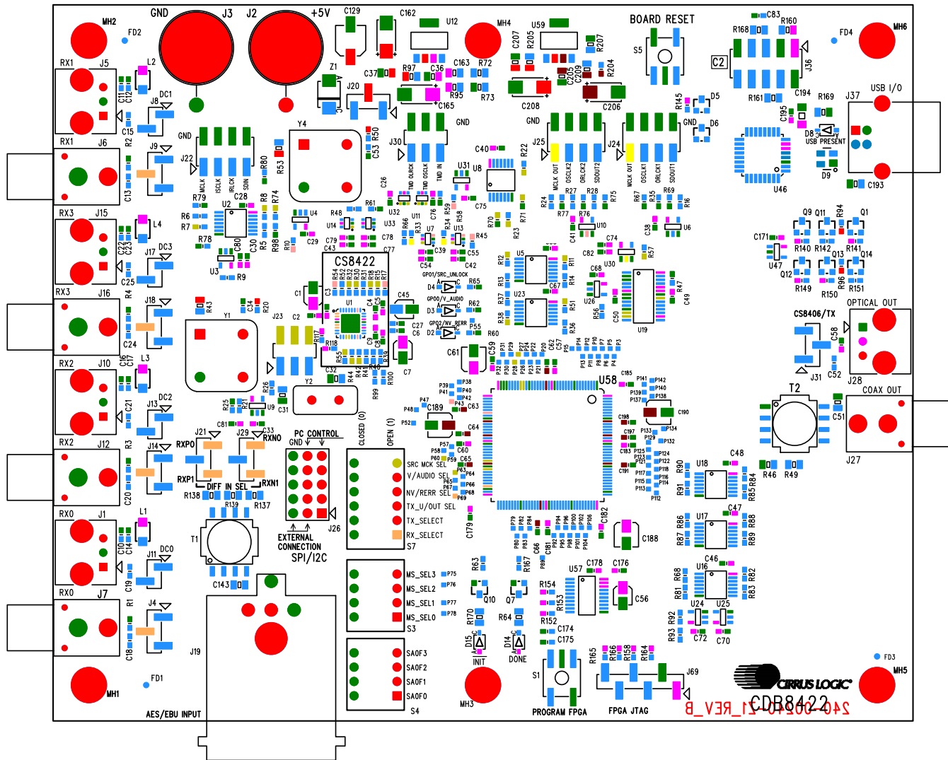
Figure 27. Silk Screen
