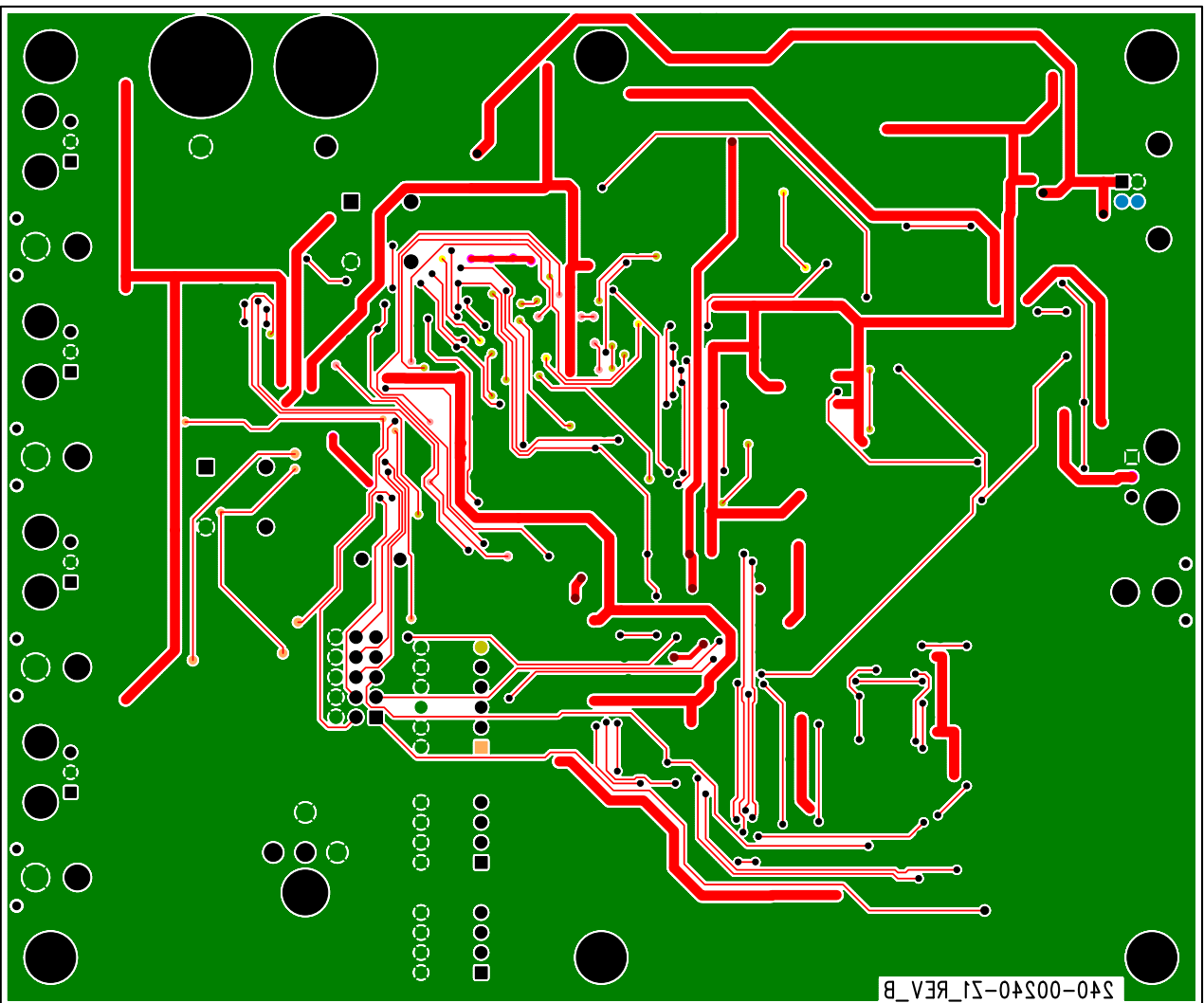
Figure 29. Bottom-Side Layer
