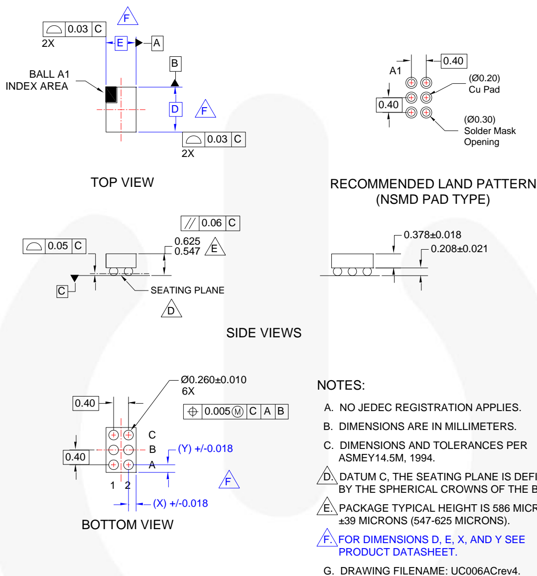
Figure 36. 6-Bump WLCSP, 0.4 mm Pitch
