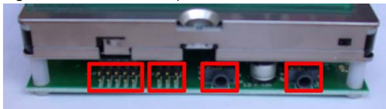
Figure 2-2. Audio and touch panel connectors
