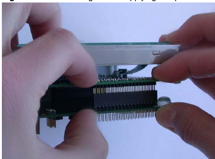
Figure 3-4. Headers aligned and applying firm pressure
