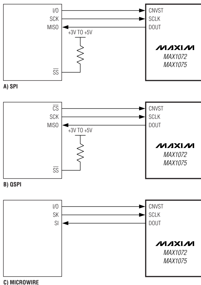
Figure 11. Common Serial-Interface Connections to the MAX1072/MAX1075
