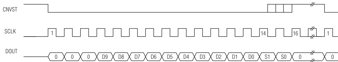
Figure 10. Continuous Conversion with Burst/Continuous Clock
