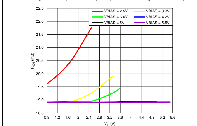
Figure 9. R ON vs. V IN (T A = 25°C, Single Channel)
