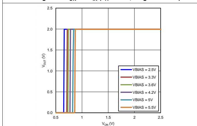
Figure 11. V OUT vs. V ON (T A = 25°C, Single Channel)
