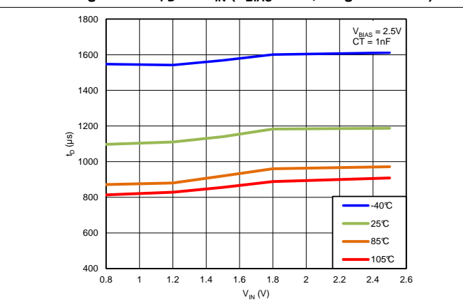
Figure 12. t D vs. V IN (V BIAS = 2.5 V, CT = 1 nF)
