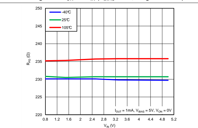
Figure 10. R PD vs. V IN (V BIAS = 5 V, Single Channel)
