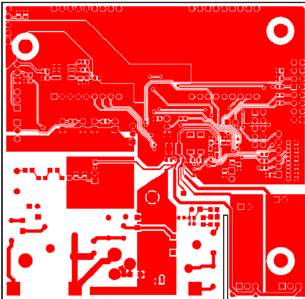
Figure 4-8: 71M6531N12A2 Demo Board: Bottom Copper Layer – Layer View from Top
