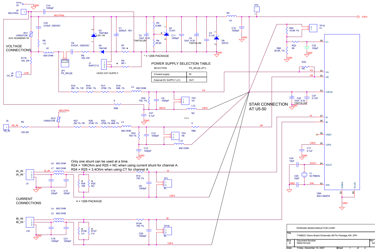
Figure 4-1: 71M6531N12A2 Demo Board (REV 2.0): Electrical Schematic 1/3 – Shunt Configuration
