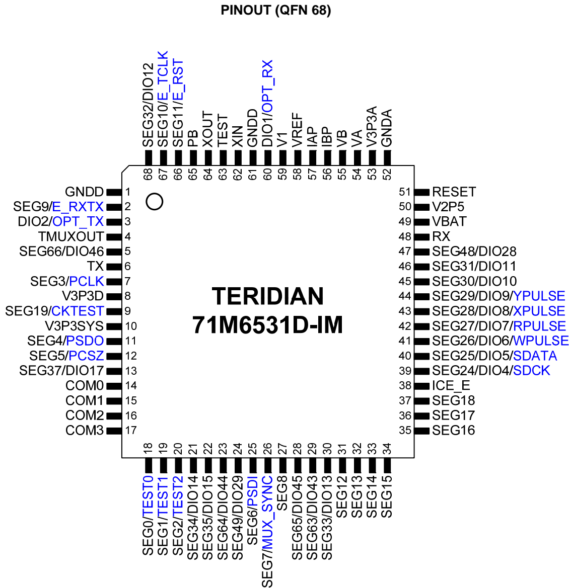
Figure 4-16: TERIDIAN 71M6531D/F LQFP64: Pinout (top view)
