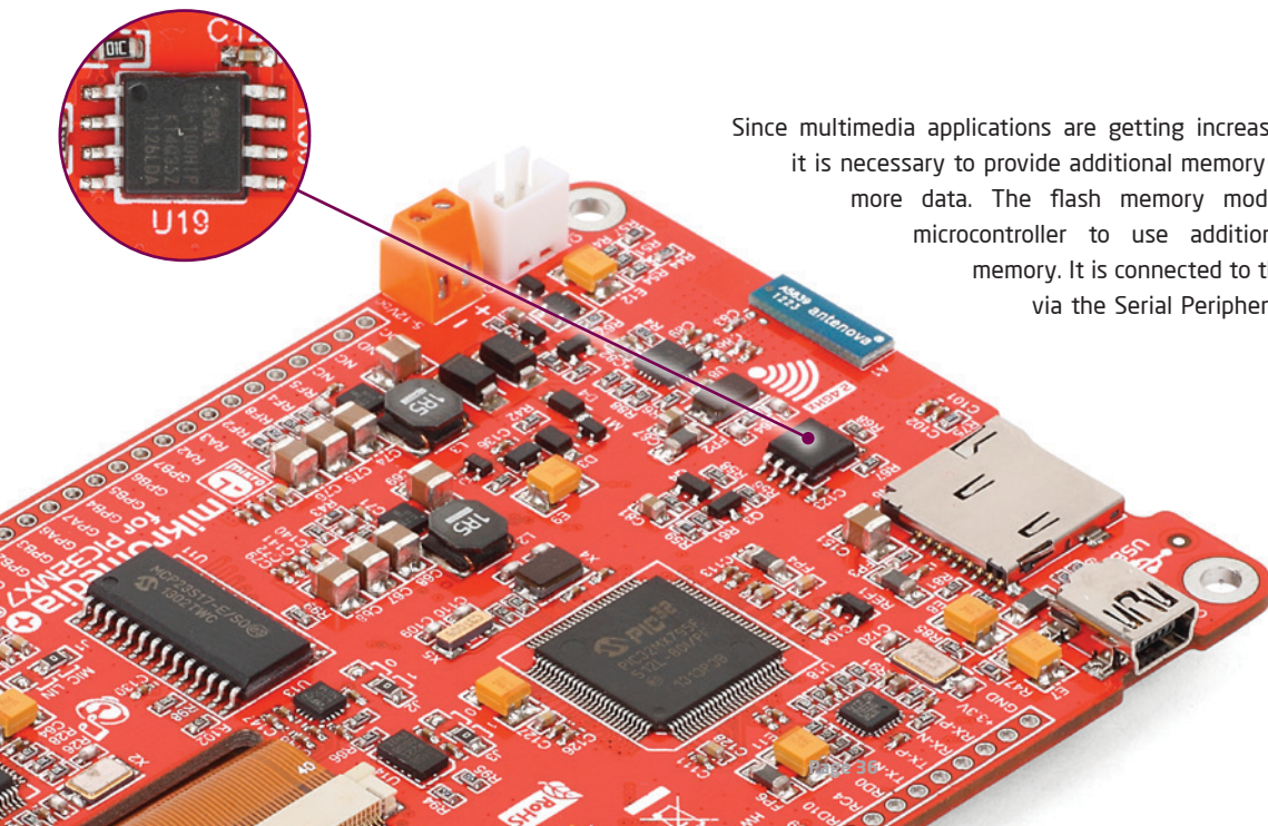
Figure 13-1: Flash memory module
