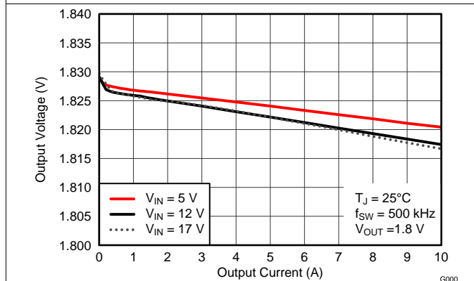
Figure 40. Load Regulation
