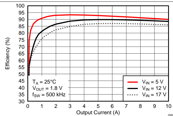
Figure 41. Efficiency
