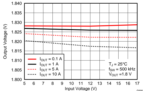
Figure 39. Line Regulation
