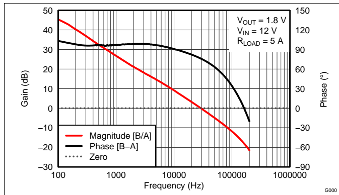
Figure 38. Closed-Loop Bode Response
