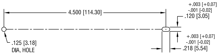
SUGGESTED MOUNTING DETAIL
