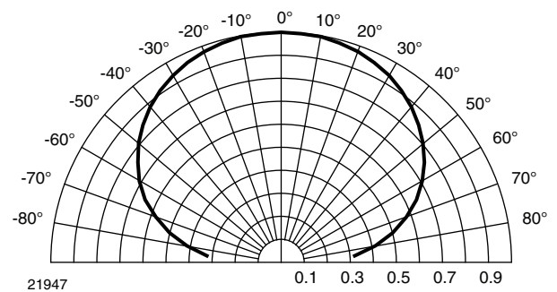
Fig. 8 - Horizontal Directivity
