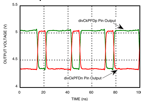
Figure 6. Time Domain 35 MHz Output, 6.5 GHz Input [4]
