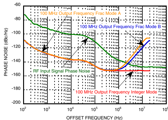
Figure 2. Output Phase Noise, 6 GHz Input Frequency [2]
